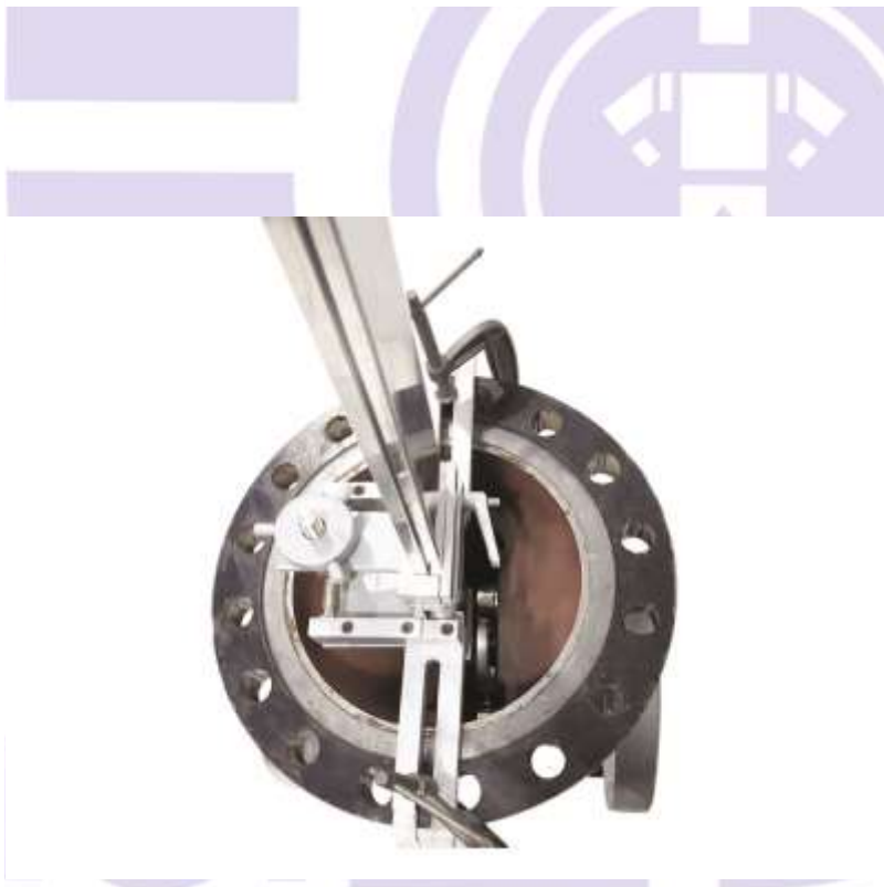
Body Seat Lapping
